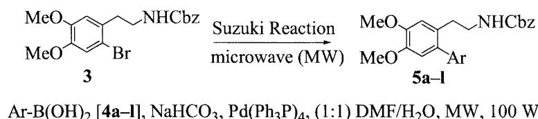
Scheme 2. Suzuki–Miyaura cross-coupling of the phenethylamine 3 with various boronic acids 4a–l
