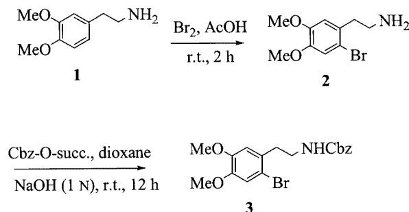
Scheme 1. Synthesis of benzyl [2-(2-bromo-4,5-dimethoxyphenyl)ethyl]carbamate ( 3 )
