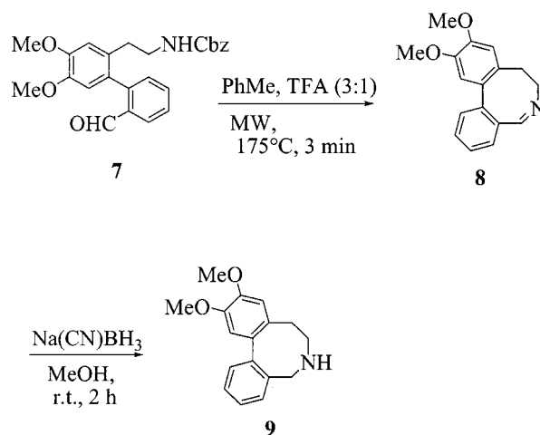
Scheme 4. Ring closure of the biaryl 7 to the Apogalanthamine analogue 9
