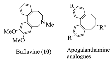
Figure 1. Apogalanthamine analogues and Buflavine ( 10 )
