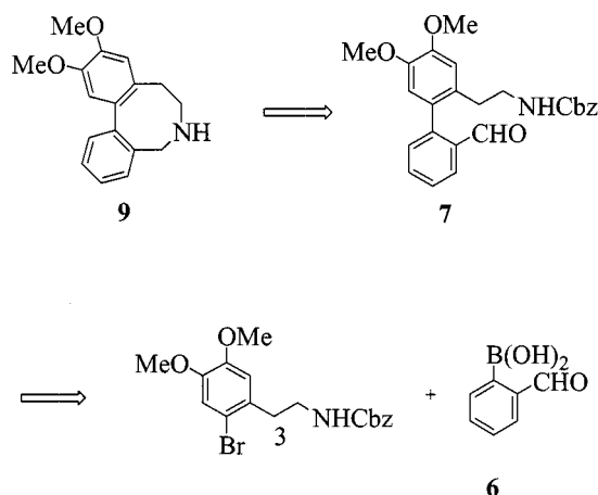
Scheme 3. Retrosynthetic analysis for the generation of 9
